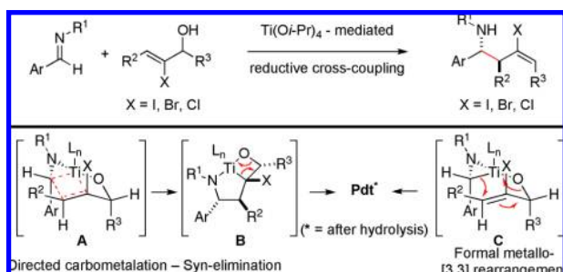
Figure 3. Imine–allylic alcohol coupling reaction.
