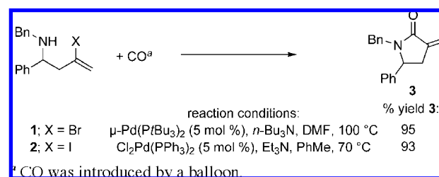
Figure 4. Pd-catalyzed carbonylative cyclization.
