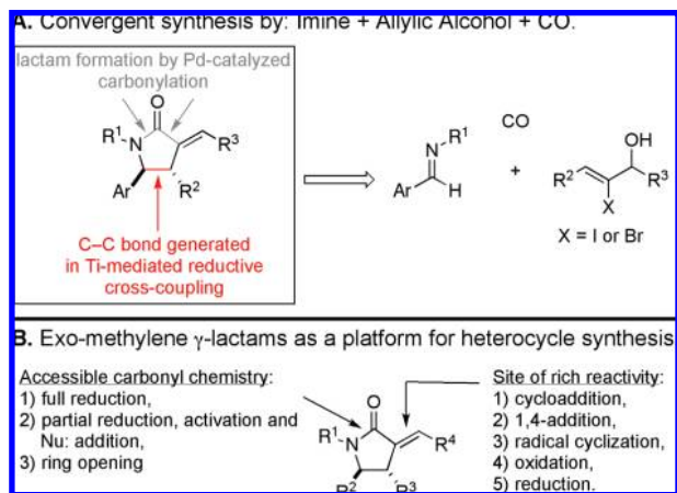
Figure 2. exo -Alkylidene- \gamma -lactams.
