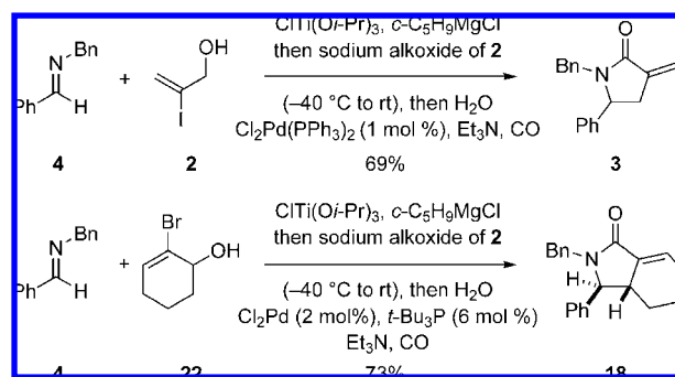
Figure 5. One-pot, three-component coupling for heterocycle synthesis.
